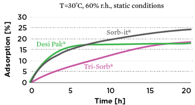
4. Adsorption rate at high RH
