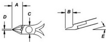
2897EHT 4-1/4" Medium Round Head Cutter with Carbide Insert
